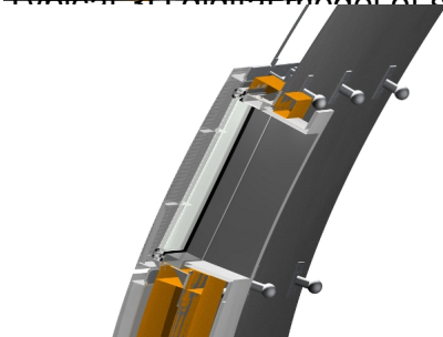
Typical 3D digital model of system development
